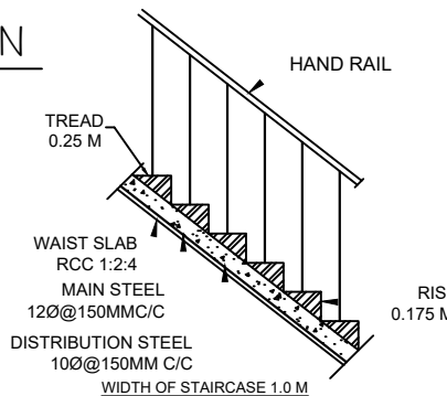
STAIR CASE DETAILS SCALE 1:300
