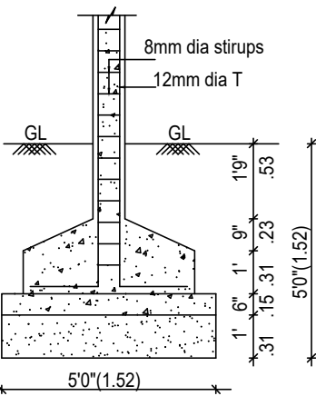
COLUMN FOUNDATION DETAIL SCALE 1"=4'0"(1:50)
