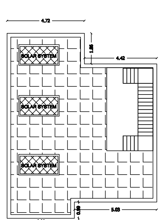
TEERACE PLAN
