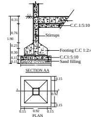
FOUNDATION DETAILS
