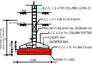
FOUNDATION DETAIL
