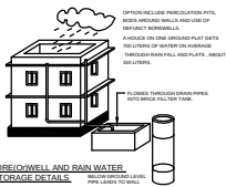
BOREWELL AND RAIN WATER STORAGE DETAILS
