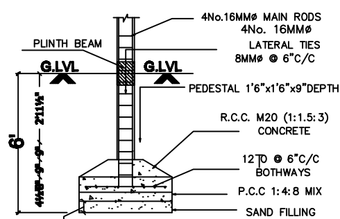
FOUNDATION DETAIL [SCALE: 1:50]
