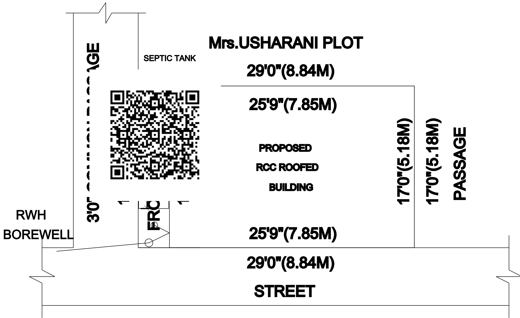
SITE PLAN
