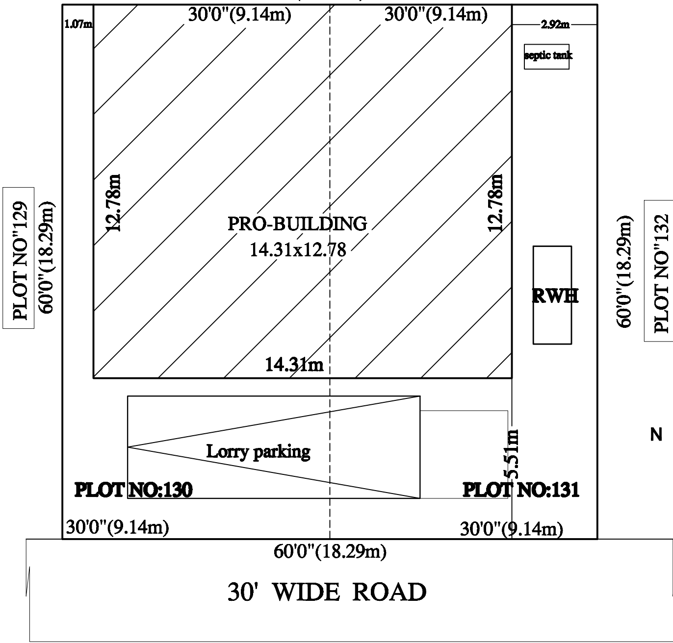
SITE PLAN
