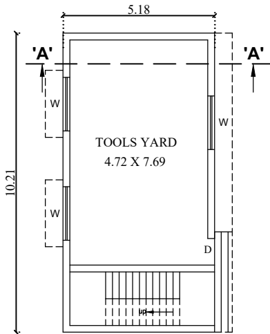
GROUND FLOOR PLAN BLOCK No. 1
