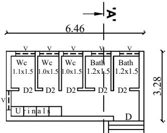
GROUND FLOOR PLAN BLOCK No.3
