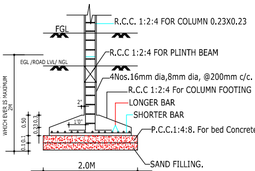
FOUNDATION DETAIL
