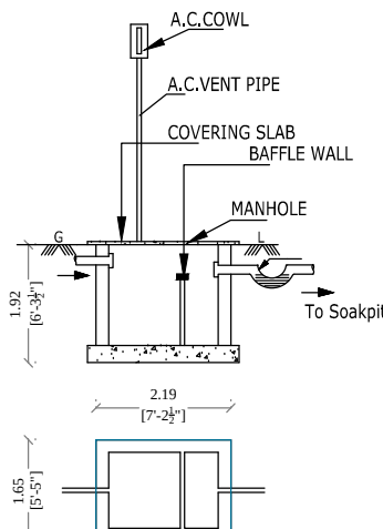
SEPTIC TANK
