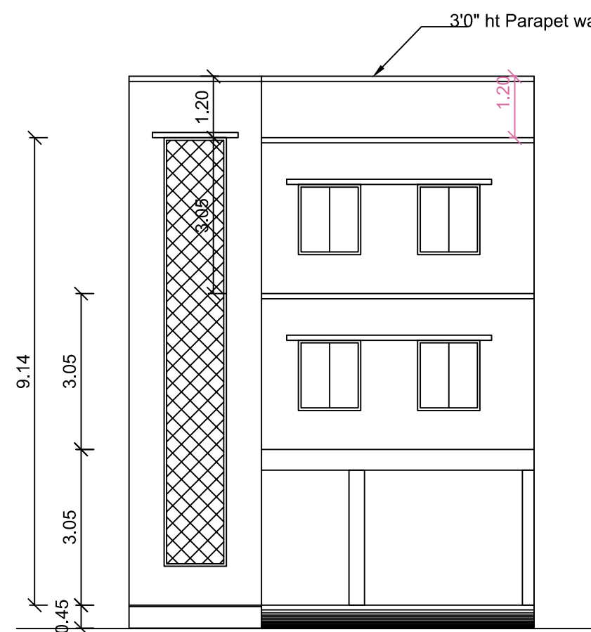
FRONT ELEVATION
