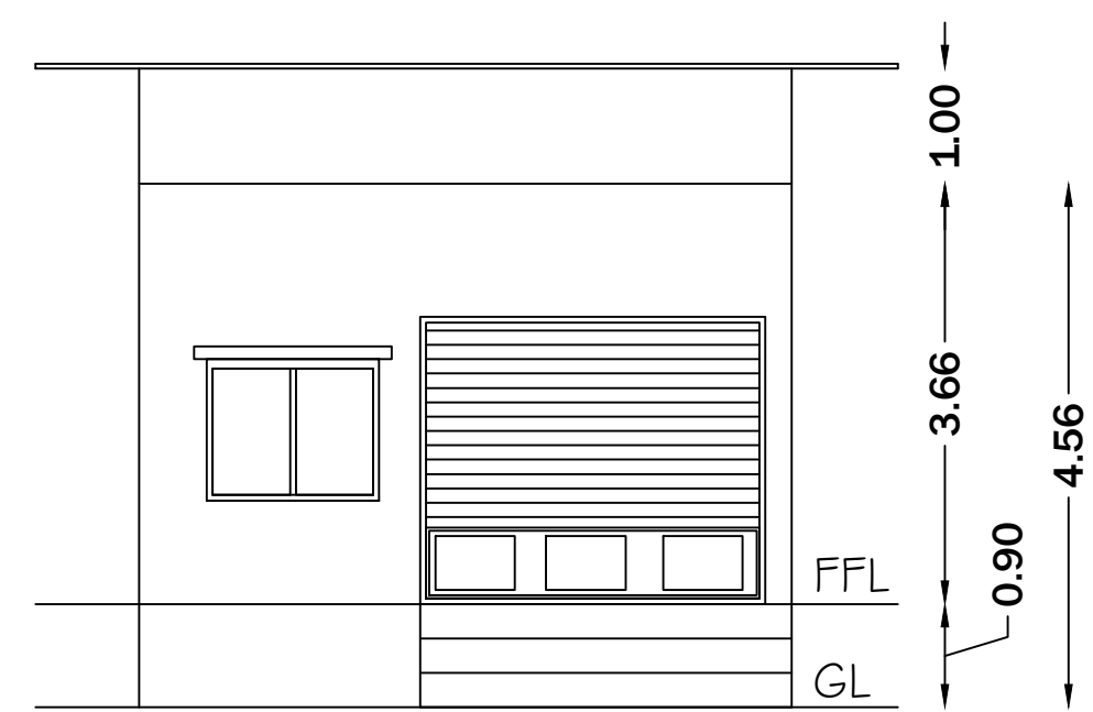
FRONT ELEVATION
