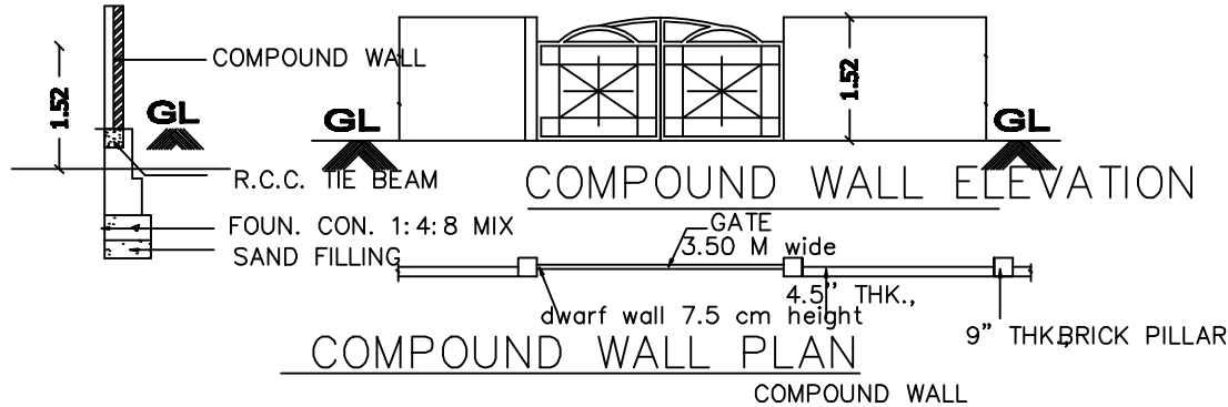
COMPOUND WALL
