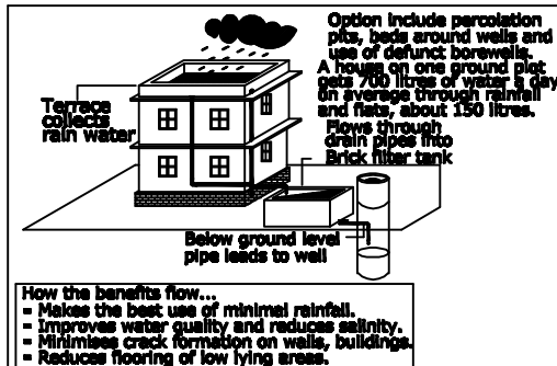
WELL AND RAIN WATER HARVEST SYSTEM
