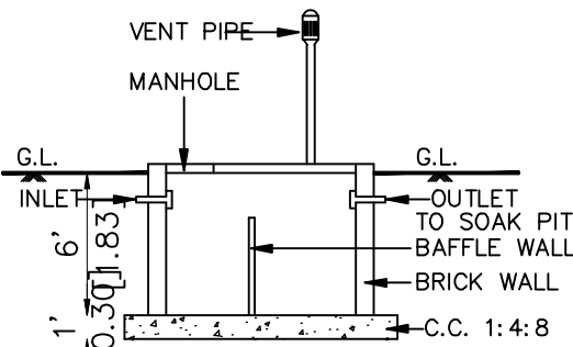
SECTION OF SEPTIC TANK
