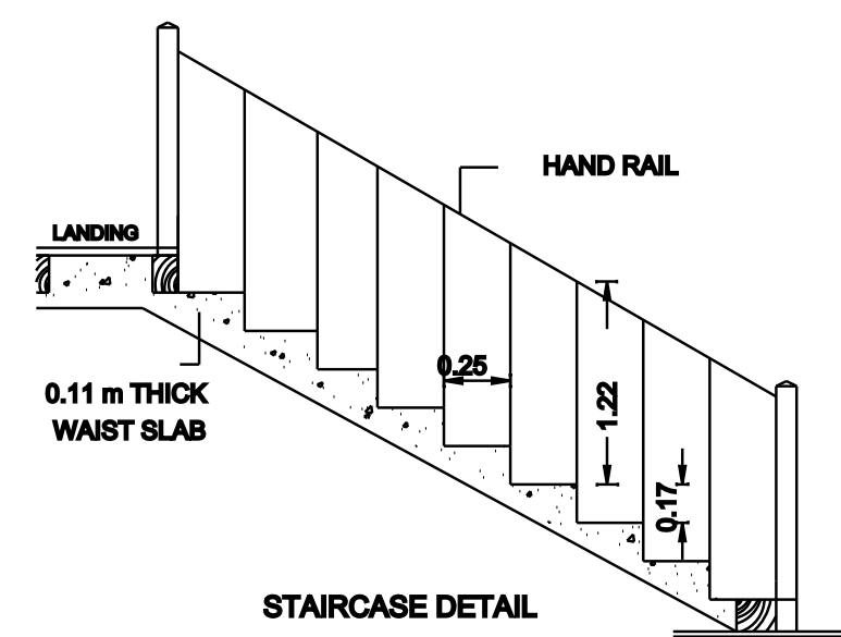
STAIRCASE DETAIL
