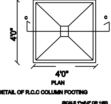
PLAN DETAIL OF R.C.C COLUMN FOOTING
