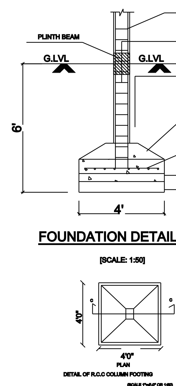
PLAN DETAIL OF R.C.C COLUMN FOOTING
