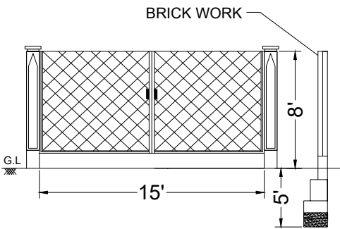
COMPOUND WALL DETAILS
