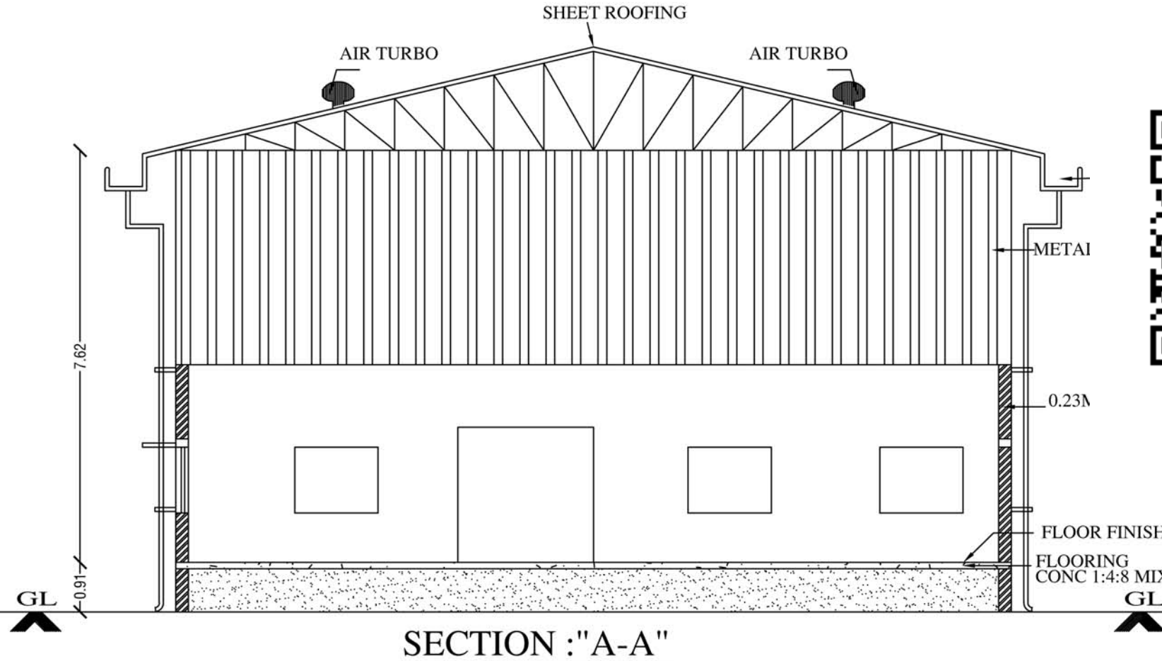
SECTION : "A-A"
