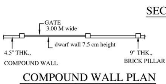
COMPOUND WALL DETAILS
