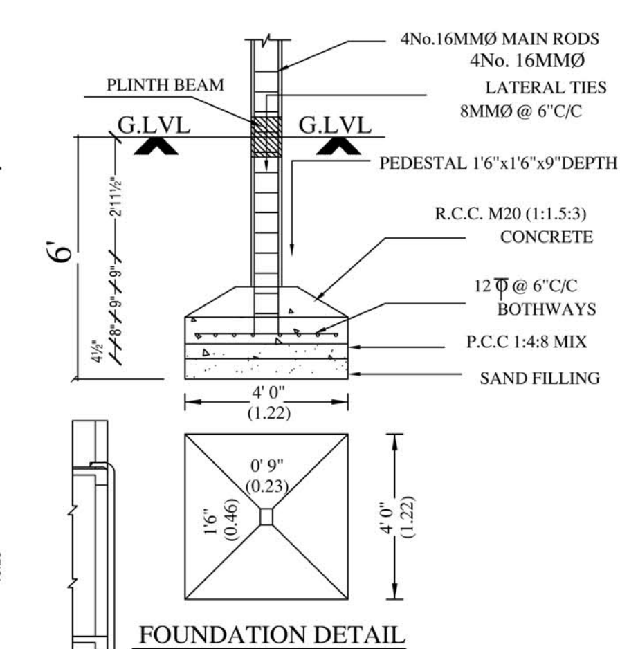
FOUNDATION DETAIL
