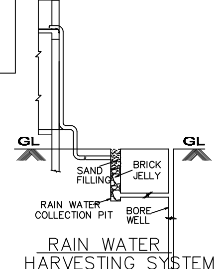
WELL AND RAIN WATER HARVEST SYSTEM
