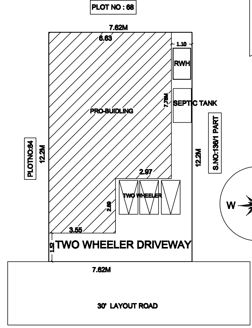
SITE PLAN
