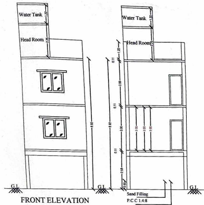
CROSS SECTION ON AB
