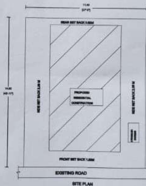
SITE PLAN
