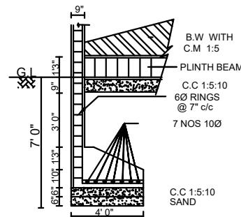
FOUNDATION DETAILS SCALE : 1/4 INCHES TO A FOOT
