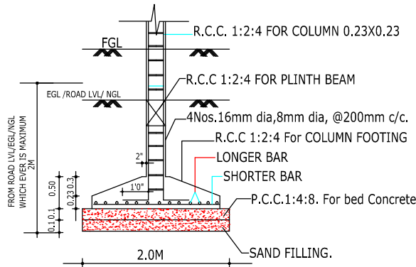
FOUNDATION DETAIL
