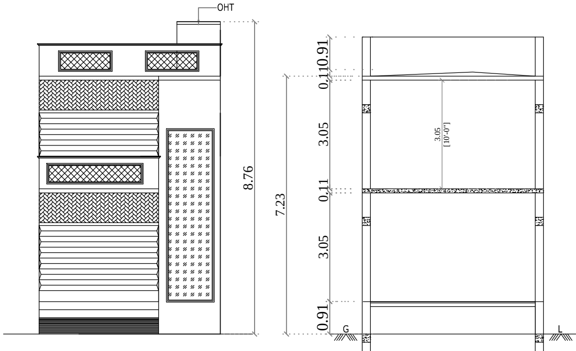
FRONT ELEVATION
