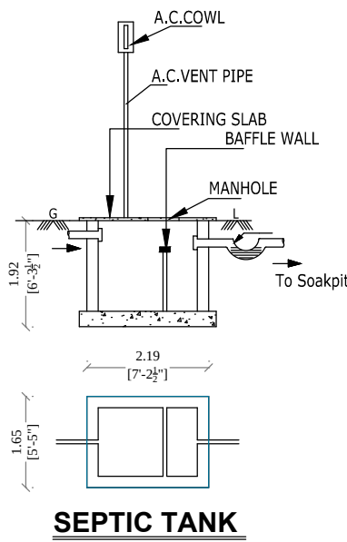
SEPTIC TANK
