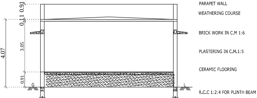
SECTION ON "SC"
