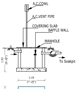
SEPTIC TANK
