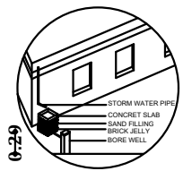
DETAIL RAINWATER HARVESTING
