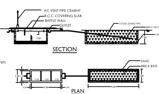
SECTION PLAN SEPTIC TANK AND TRENCH
