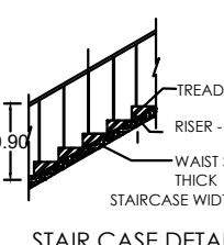
STAIR CASE DETAIL
