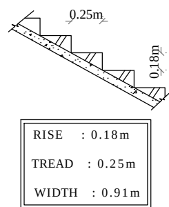
STAIRS DETAILS
