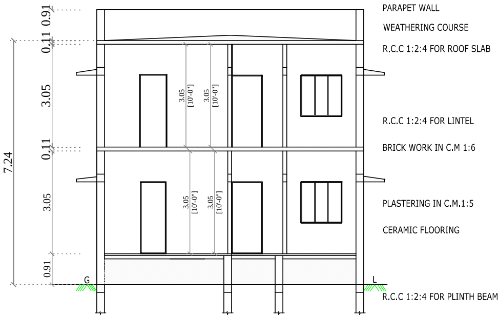
SECTION ON "SC"
