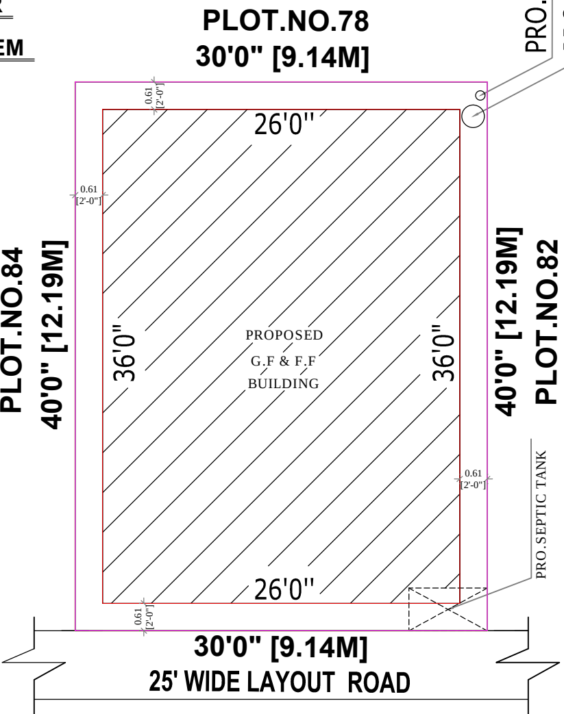
SITE PLAN SCALE: 1 INCH = 16 FEET
