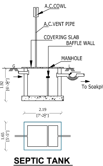
SEPTIC TANK
