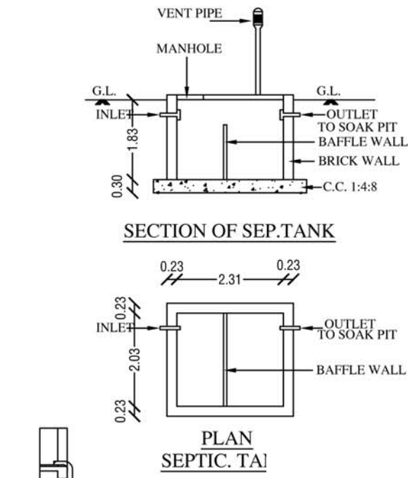
SECTION OF SEP. TANK
