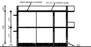
SECTION ON " MS "
