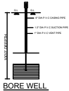
BORE WELL
