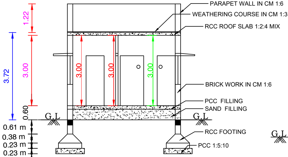
SECTION OF "A-A"
