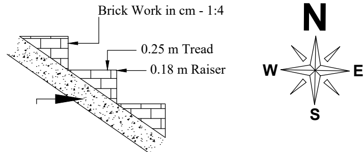
STAIR CASE DETAILS (Scale 1 : 1)
