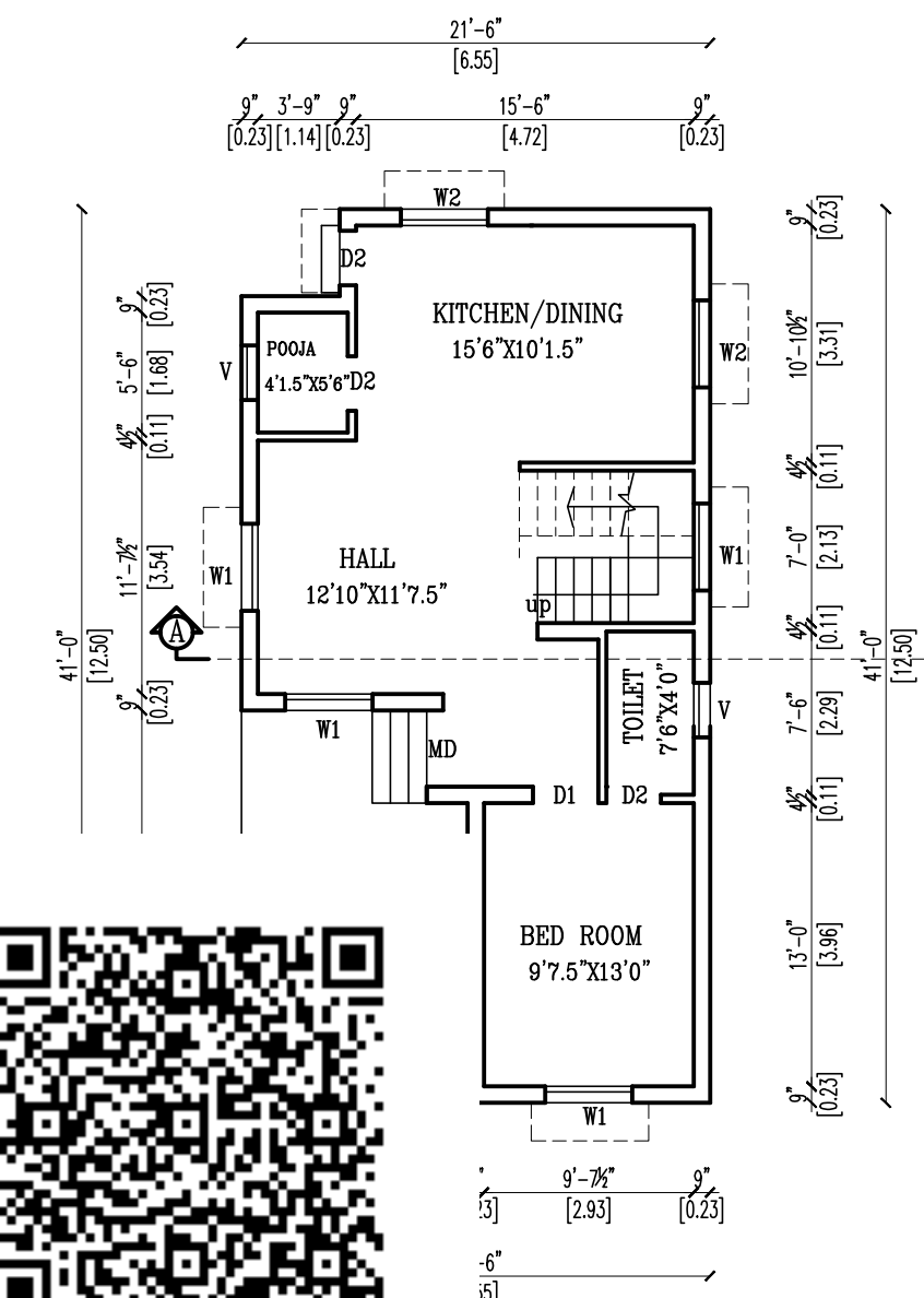
ND FLOOR PLAN
