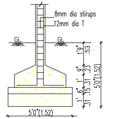
COLUMN FOUNDATION DETAIL SCALE 1":4'0"(1:50)
