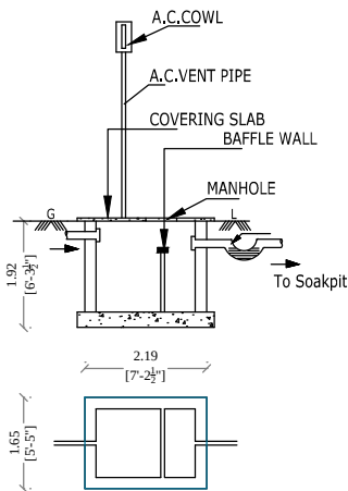
SEPTIC TANK
