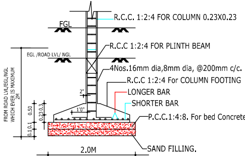
FOUNDATION DETAIL
