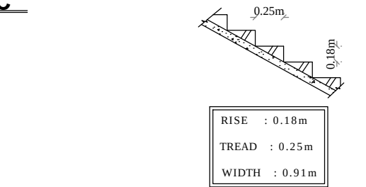
STAIRS DETAILS
