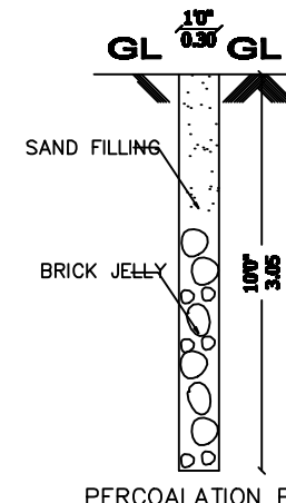
PERCOALATION PIT
