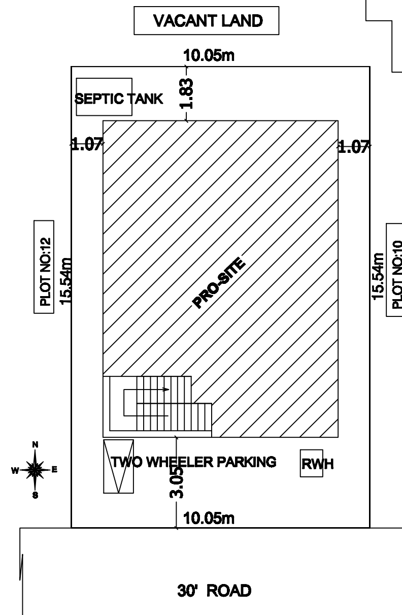
SITE PLAN
