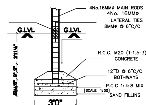
FOUNDATION DETAIL
