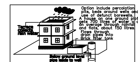
WELL AND RAIN WATER HARVEST SYSTEM
