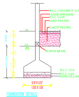
FOUNDATION DETAILS
