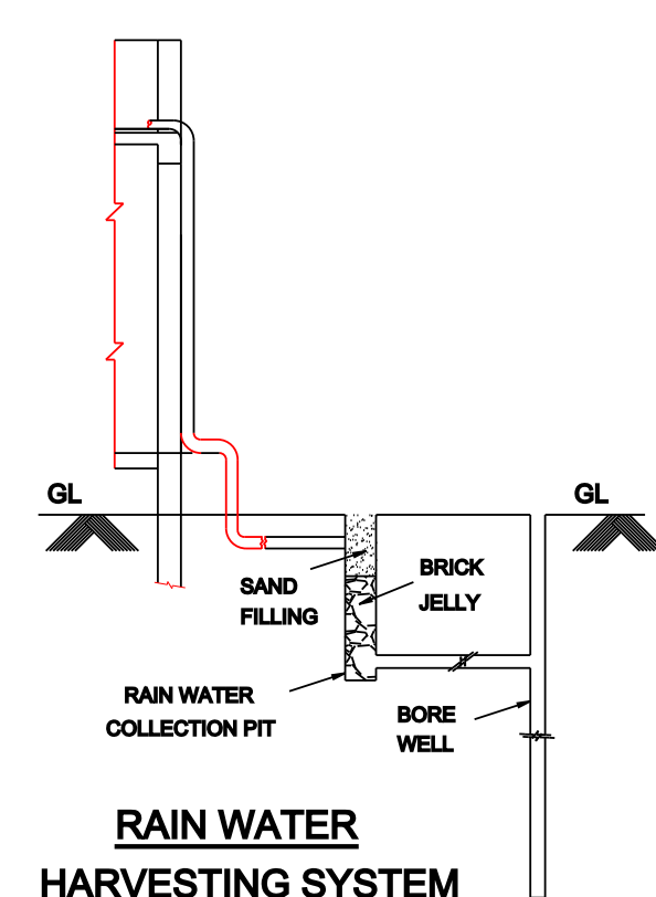
RAIN WATER HARVESTING SYSTEM
