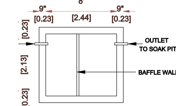
PLAN SEPTIC. TANK
