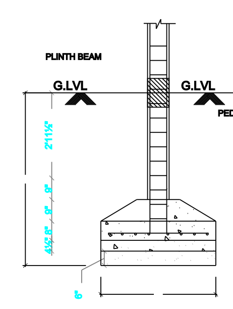
FOUNDATION DETAIL
