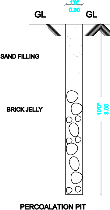
PERCOLATION PIT
