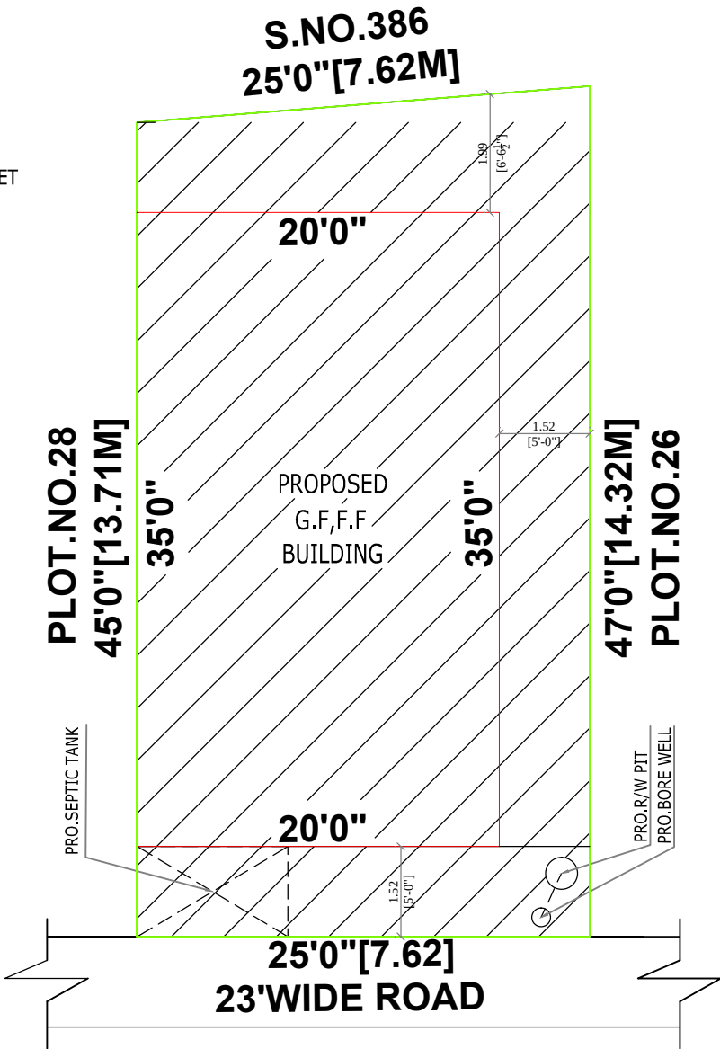
SITE PLAN SCALE: 1 INCH = 16 FEET
