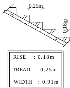
STAIRS DETAILS
