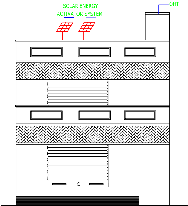
FRONT ELEVATION
