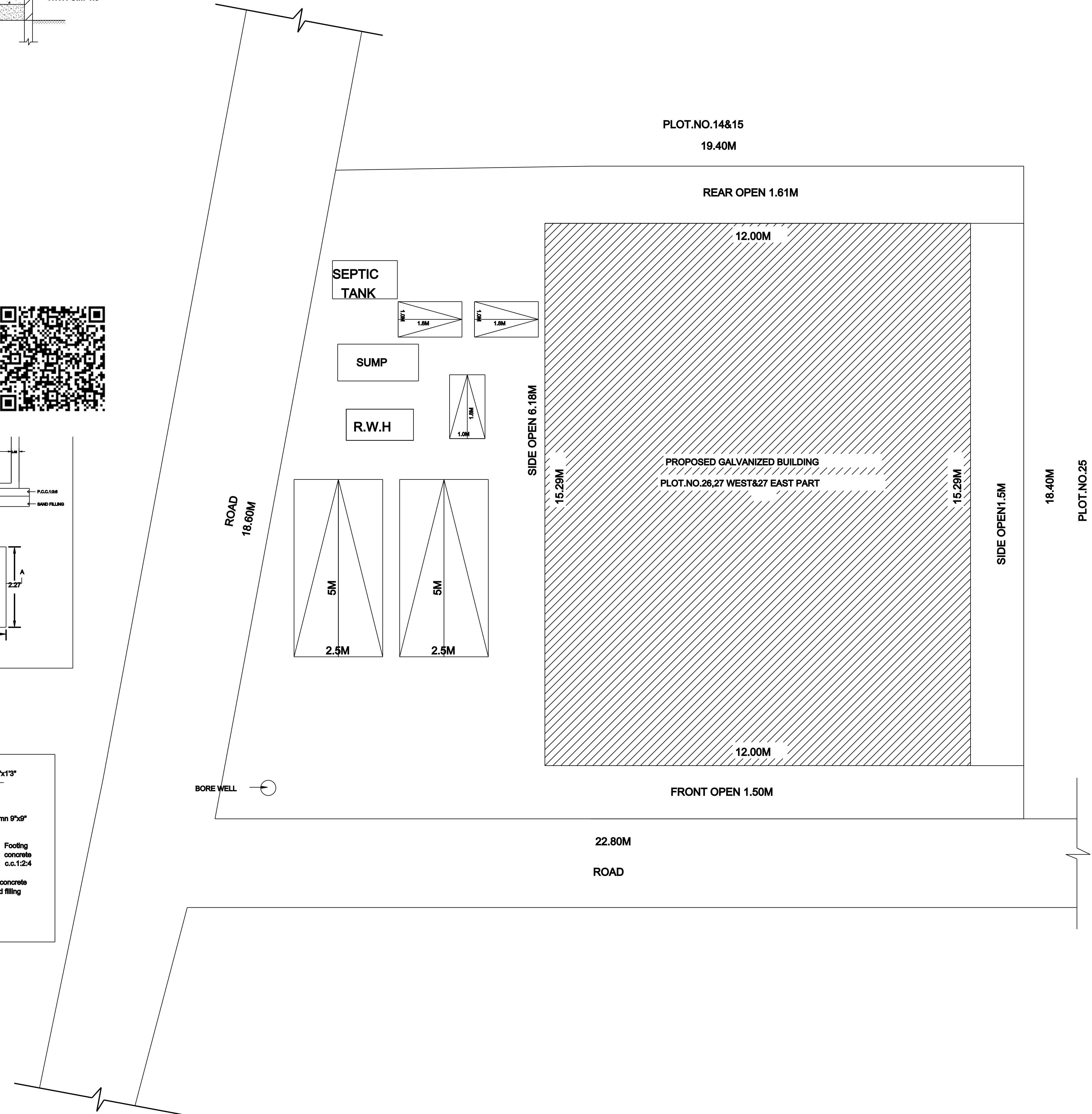
KEY PLAN
