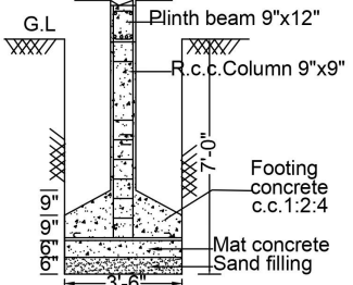
FOUNDATION DETAILS (SCALE : 1" = 4'-0")
