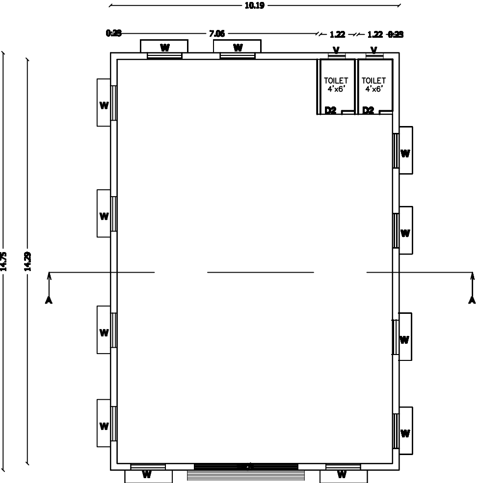
PLAN
