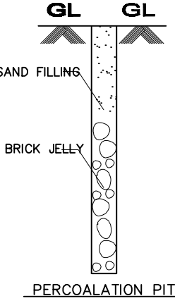
PERCOLATION PIT
