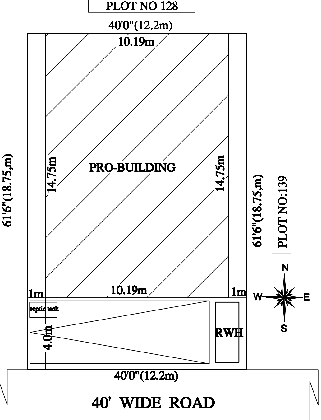
SITE PLAN
