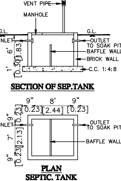
PLAN SEPTIC TANK
