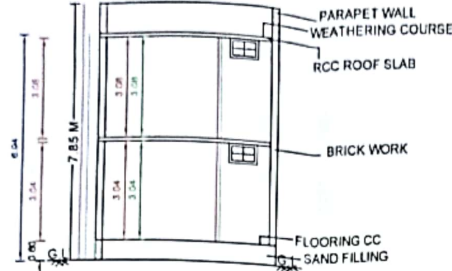
FLOOR SECTION ON S.B
