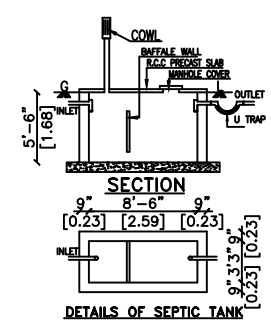
DETAILS OF SEPTIC TANK
