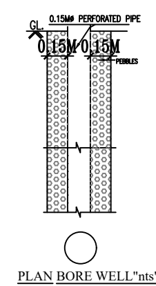
PLAN BORE WELL "mts"
