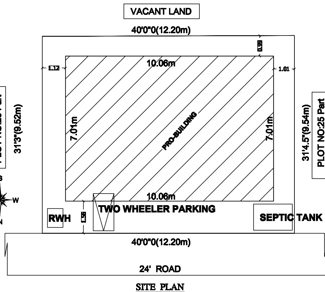
SITE PLAN
