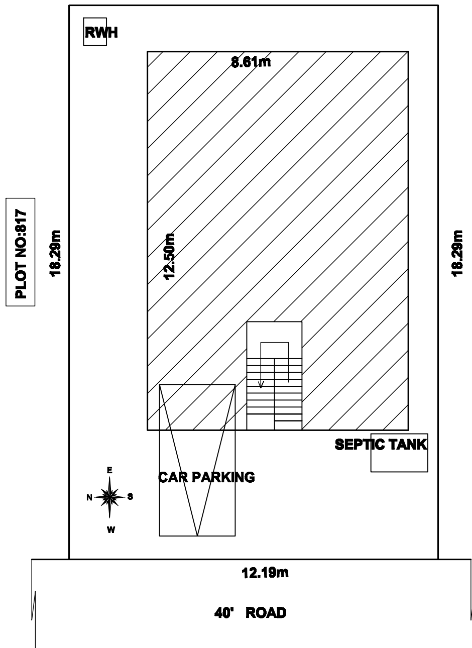
SITE PLAN
