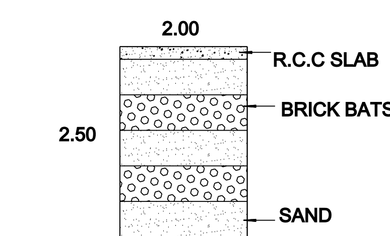
SECTION ON C - D
