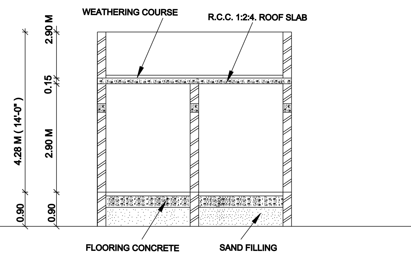
SECTION ON " MS "
