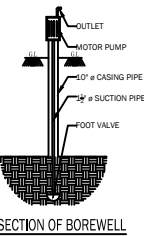
SECTION OF BOREWELL
