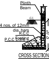
CROSS SECTION
