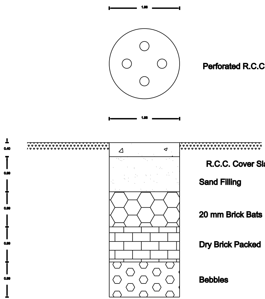
RAIN WATER HARVESTING (Scale 1 : 1)
