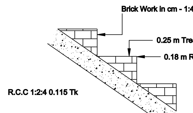
STAIR CASE DETAILS (Scale 1 : 1)
