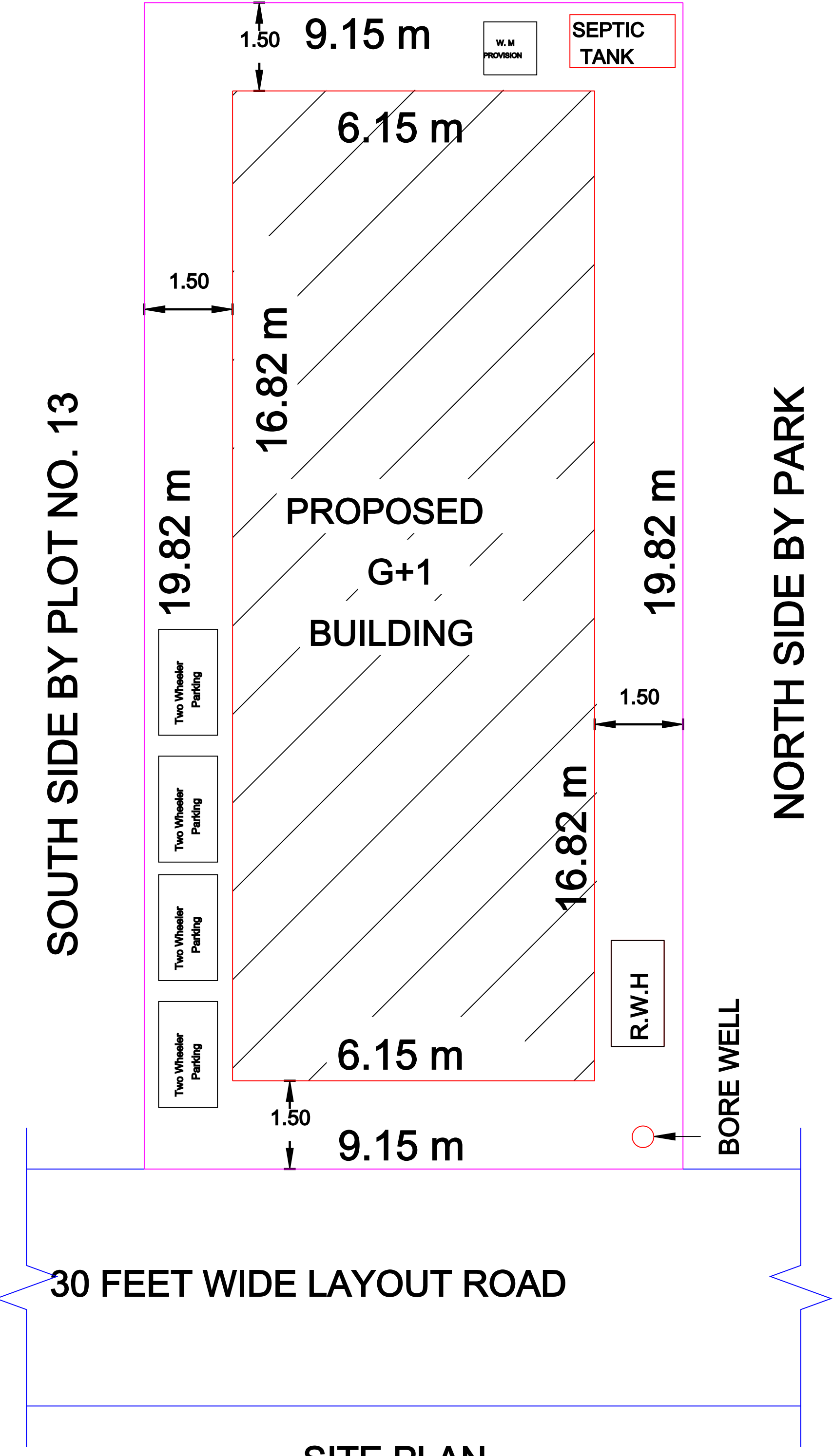
SITE PLAN
