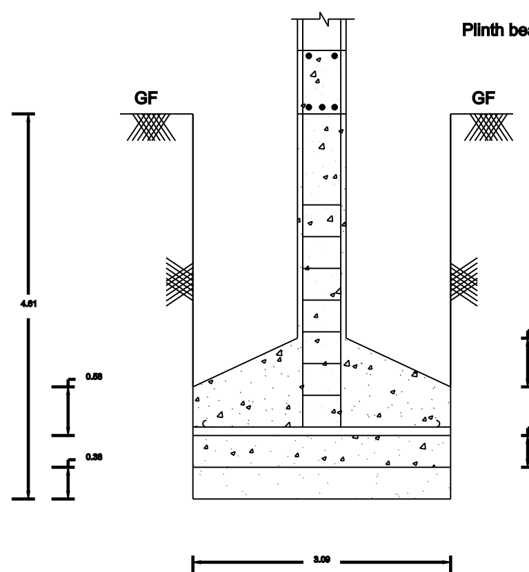
FOUNDATION DETAILS (Scale 1 : 1)
