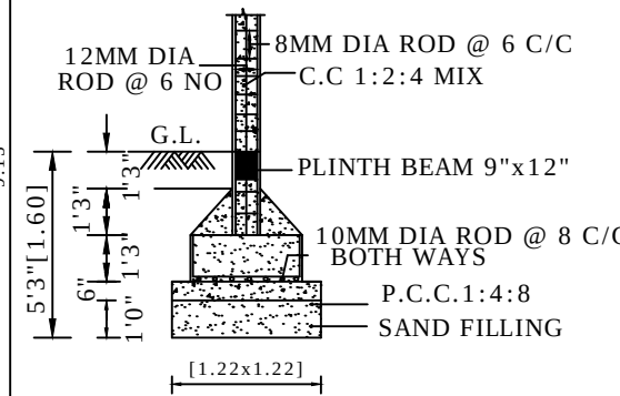
RUN THROUGH COLUMN FOUNDATION SCALE 1"=4'0" (1:50)
