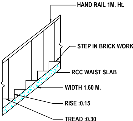
STAIR DETAIL
