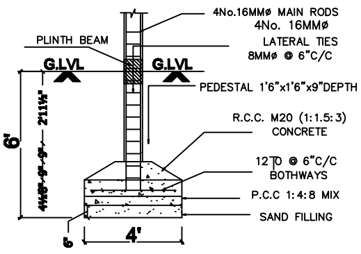
FOUNDATION DETAIL
