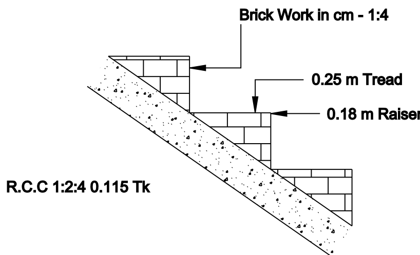
STAIR CASE DETAILS (Scale 1 : 1)
