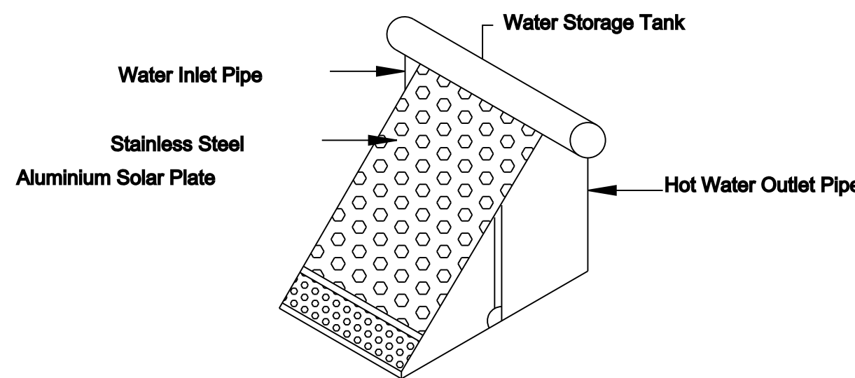
SOLAR WATER HEATER (DOMESTIC MODEL) CAPACITY 100 TO 100000 Ltrs/DAY TEMP - 90 C °
