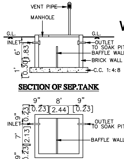
PLAN SEPTIC. TANK
