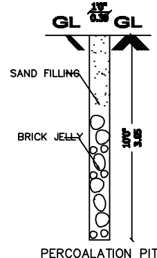
PERCOLATION PIT
